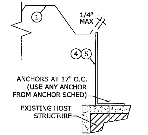
5 BUILD-OUT MOUNT CLOSURE 2 3" = 1'-0" PLAN VIEW
