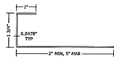
5 STEEL J-PAN CLOSURE 4" = 1'-0"
