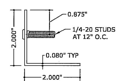
2 STUDDED ANGLE 6" = 1'-0"
