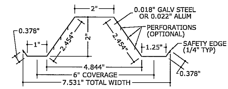
1b STEEL/ALUM HALF-PANEL PROFILE 4" = 1'-0" SECTION
