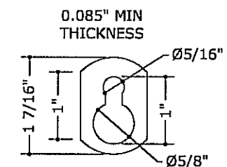
3 KEYHOLE WASHER 6" = 1'-0"
