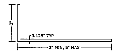
4 ALUMINUM CLOSURE 4" = 1'-0"
