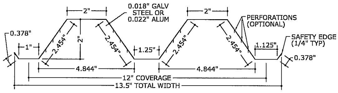
1a STEEL/ALUM STORM PANEL PROFILE 4" = 1'-0" SECTION
